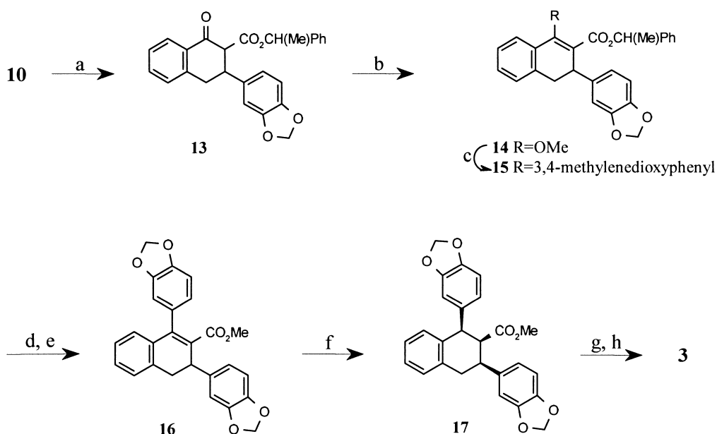
Scheme 4. Reagents: (a) \text{Ph(Me)CHOH} , DMAP, PhMe; (b) \text{CH}_2\text{N}_2 , EtOH; (c) 3,4-Methylenedioxyphenyl-magnesium bromide THF; (d) \text{H}_2 (55 psi), 5 h, EtOAc; (e) \text{CH}_2\text{N}_2 , MeOH; (f) \text{H}_2 (55 psi), 72 h, EtOAc; (g) MeONa/MeOH, THF; (h) aq NaOH/MeOH, aq HCl.
